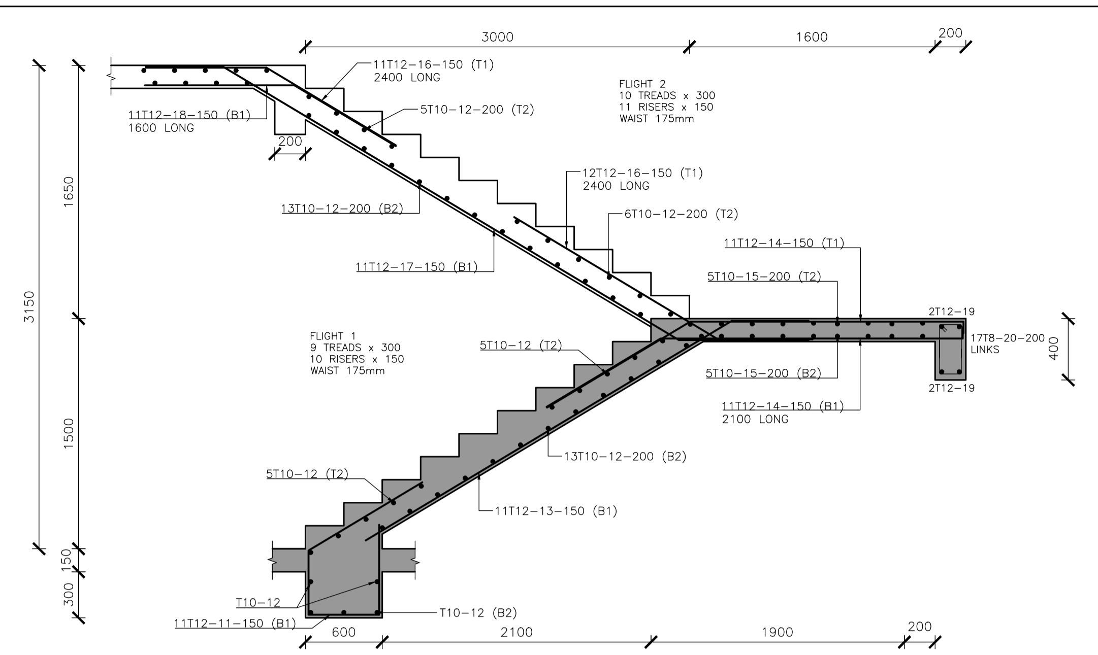
SECTION THRO' GROUND FLOOR STAIRCASE
