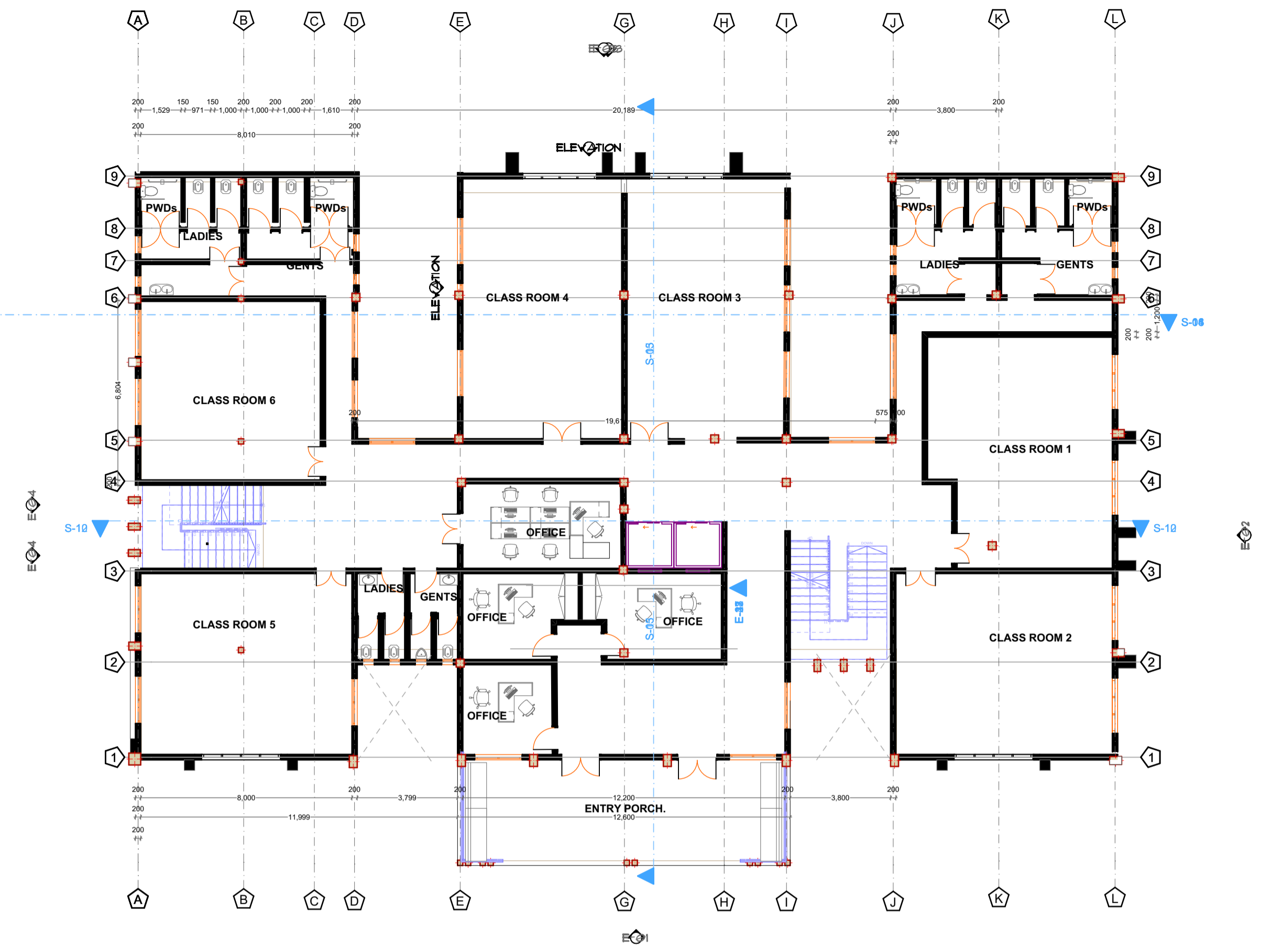
Story 1 /Story 2/story3/Story 4Typical
