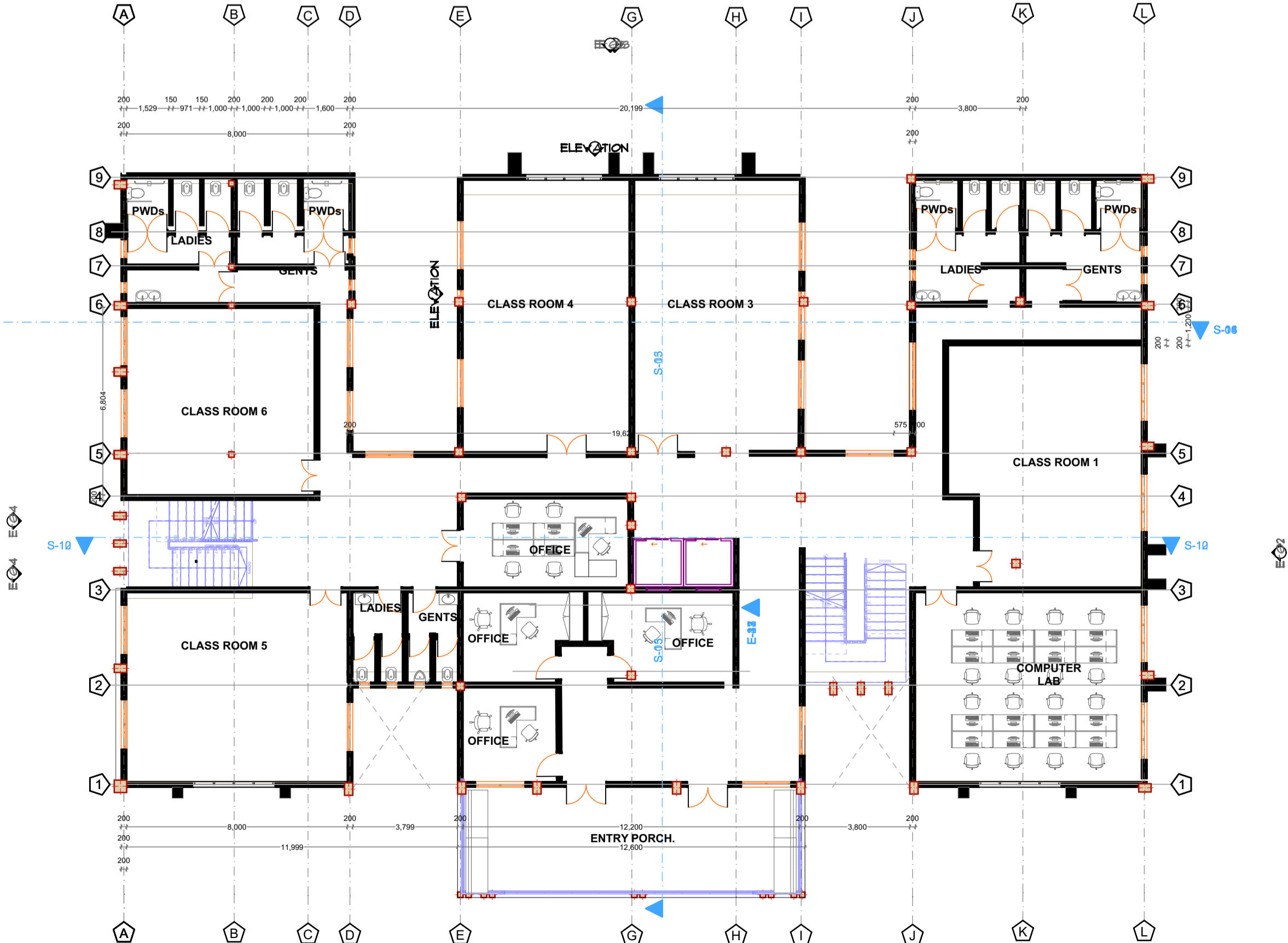
Story 5/story6 Typical
