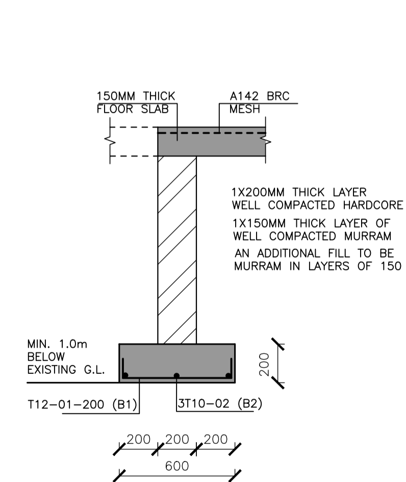
TYPICAL WALL STRIP FOOTING
