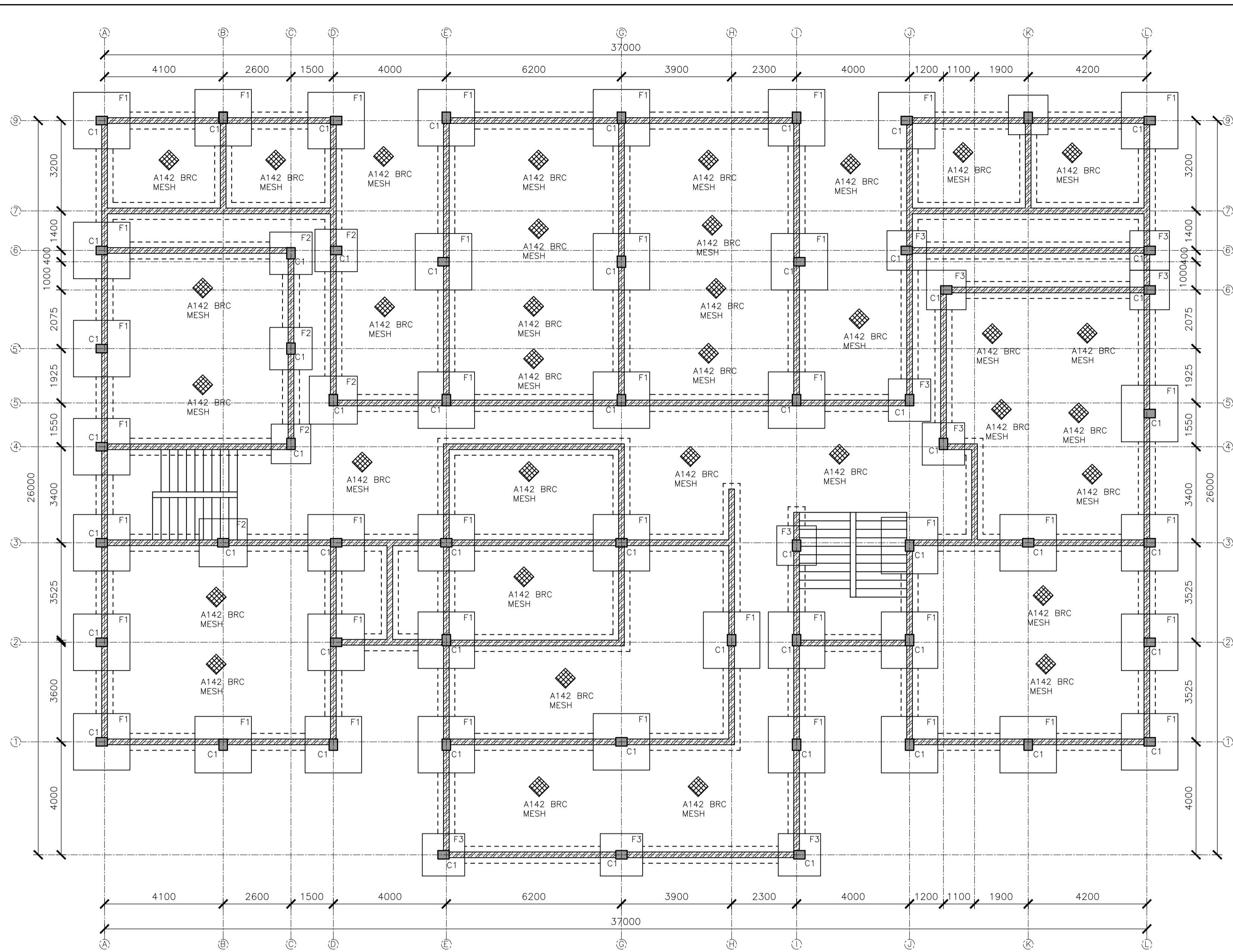
FOUNDATION LAYOUT
